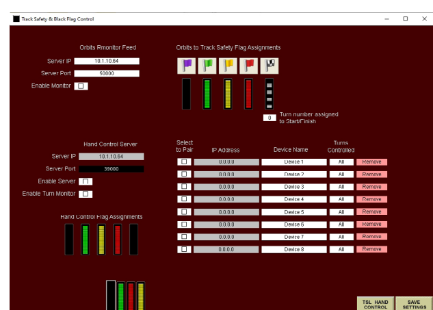
Figure 14 - Remote Control Screen
